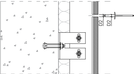
[ Fixed point ]
