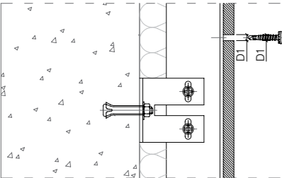
[ Fixed point ]
