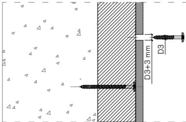
[ Floating point ]
