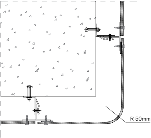
Exterior pre-curved corner
