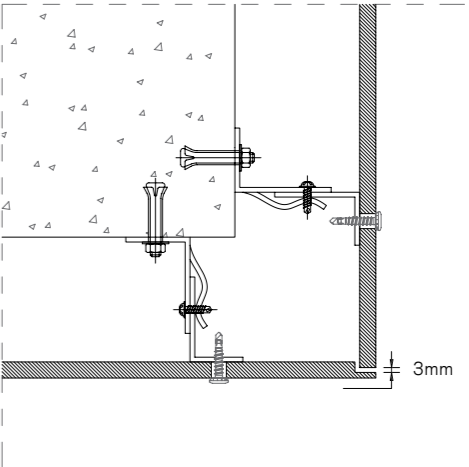
Pilaster edges
