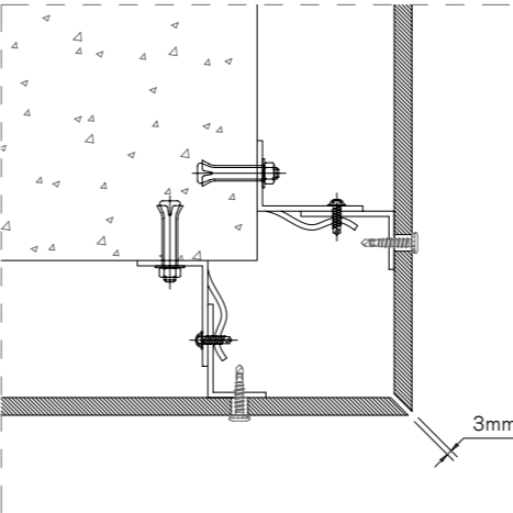
Mitered corner
