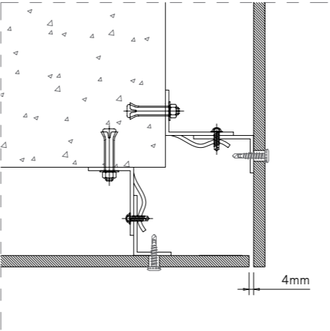
Overlapping edges
