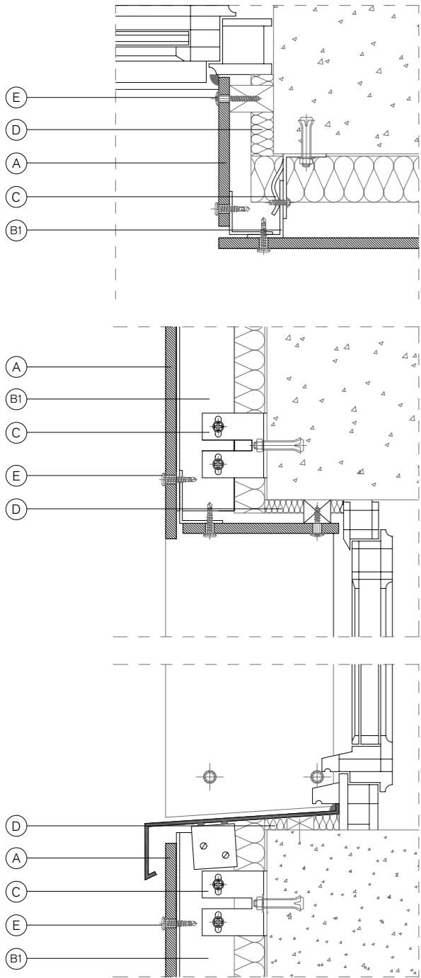
Exposed screw or rivet fixing
