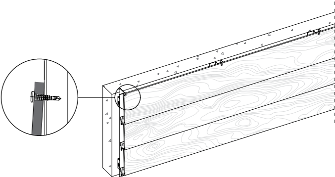
Top fixations with typical Parklex screws
