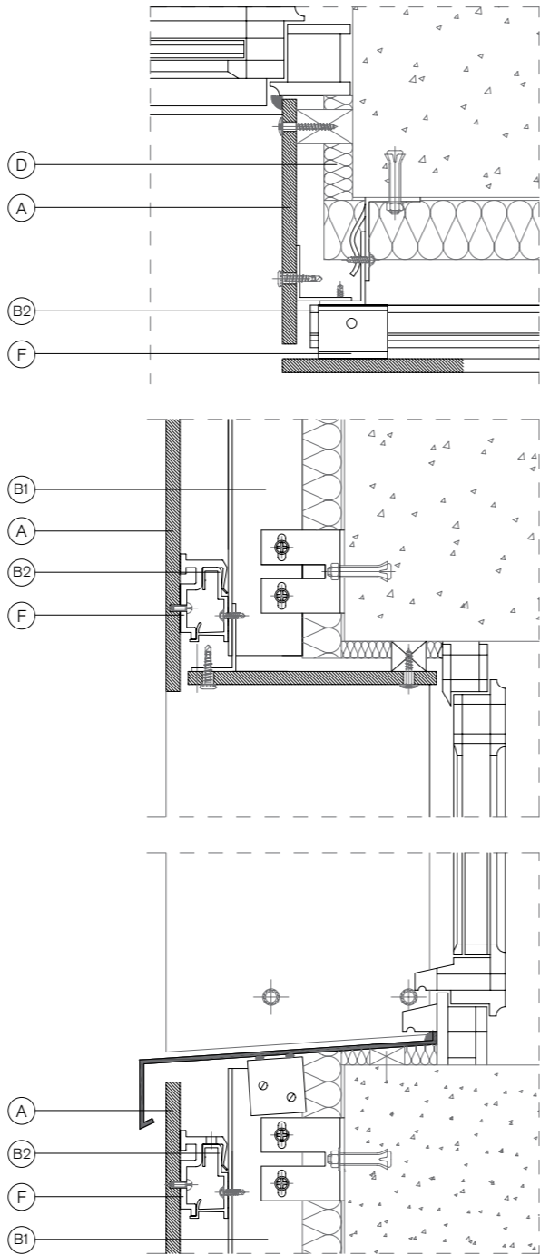
Hidden fixing with bracket hanging system
