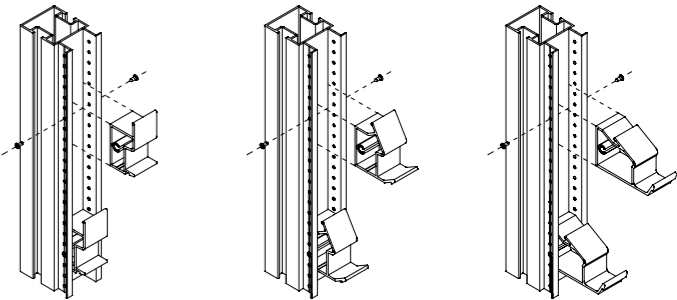
Installation of 0° Louvre base piece Installation of 30° Louvre base piece Installation of 60° Louvre base piece
