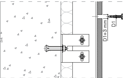
[ Floating point ]
