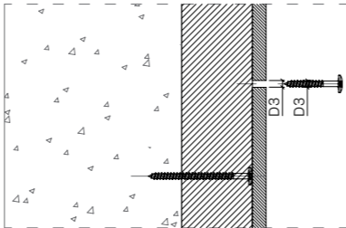
[ Fixed point ]
