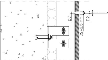
[ Floating point ]
